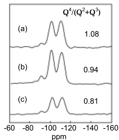
Fig. 2 Si MAS NMR spectra of as-synthesized mesoporous silica fibers prepared using various alkoxides (a) TBOS, (b) TPOS, (c) TEOS.
