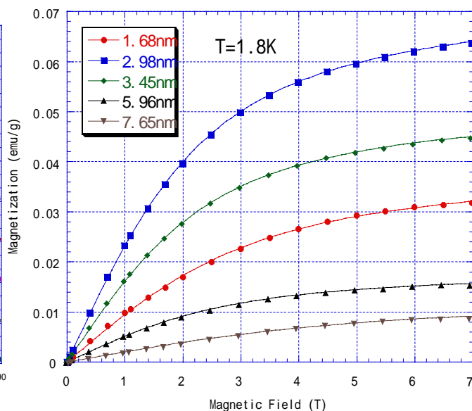
[Fig.2] Size dependence of magnetization.
