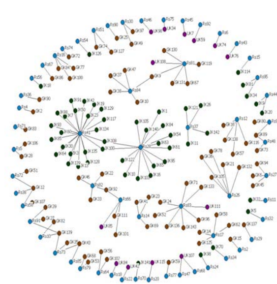
Fig.2 Researchers-keywords network
