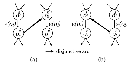
Fig. 3 Disjunctive arcs induced by functional unit assignment.
