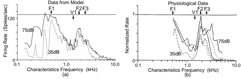
Figure 6: Rate-place representation of population of modeled and actual chopper units. (a): Data from the model. (b): Physiological data (Blackburn and Sachs, 1990).
