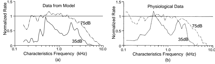
Figure 3: Rate-place representation of modeled and actual ANFs. (a): Data from the the model (High SR). (b): Physiological data (High SR) (Blackburn and Sachs, 1990). Stimulus is vowel / \epsilon / at 35 and 75 dB SPL. The line is weighting moving average whose base was 0.25 octave wide. The normalized rate defined as “rate minus SR” divided by “saturation rate minus SR”.
