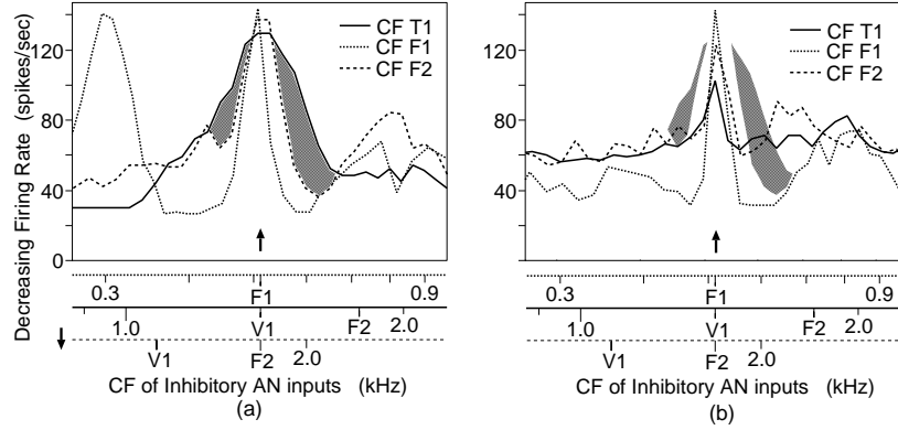
Figure 5: Responses of modeled chopper units with CF F1, F2 and V1 to the vowel / \epsilon /. Arrays show CF of models with CF F1 F2 and V1. (a): High sound level (75dB). (B): Low sound level (35dB). The method of calculation is shown in Fig.4.
