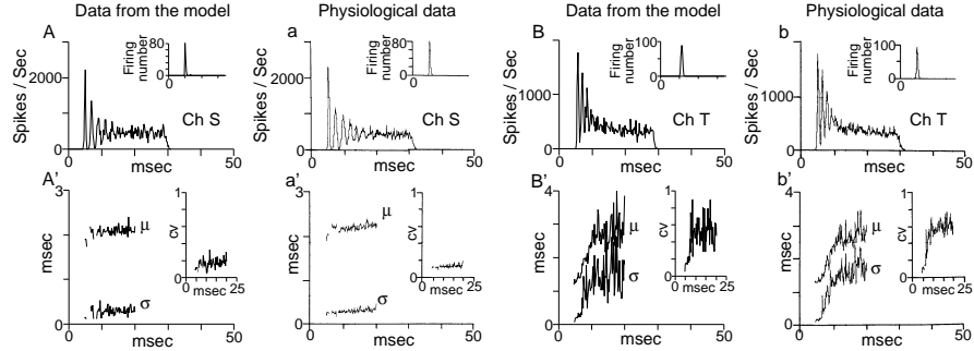
Figure 1: PSTHs (top) and regularity analysis (bottom) for Ch S and Ch T units. (A),(B): Data from the model. (a),(b): Physiological data (Blackburn and Sachs, 1990). Stimulus was 25ms STB with 1.6ms rise and fall time. PSTHs were generated from 200 presentations of the STB in the model and 300 or 500 presentations in physiological data. First-spike latency histograms are shown on the same time scale above the PSTHs. (A'),(a'),(B),(b): Regularity analysis for the data shown above. \mu is the mean inter-spike interval (ISI), \sigma is the SD of the ISI, and CV is the ratio \mu/\sigma .
