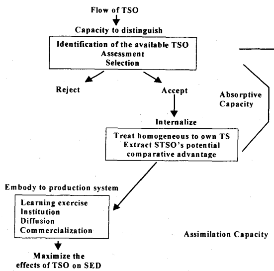
図1 The concept of assimilation capacity for spilling over technology [5]
