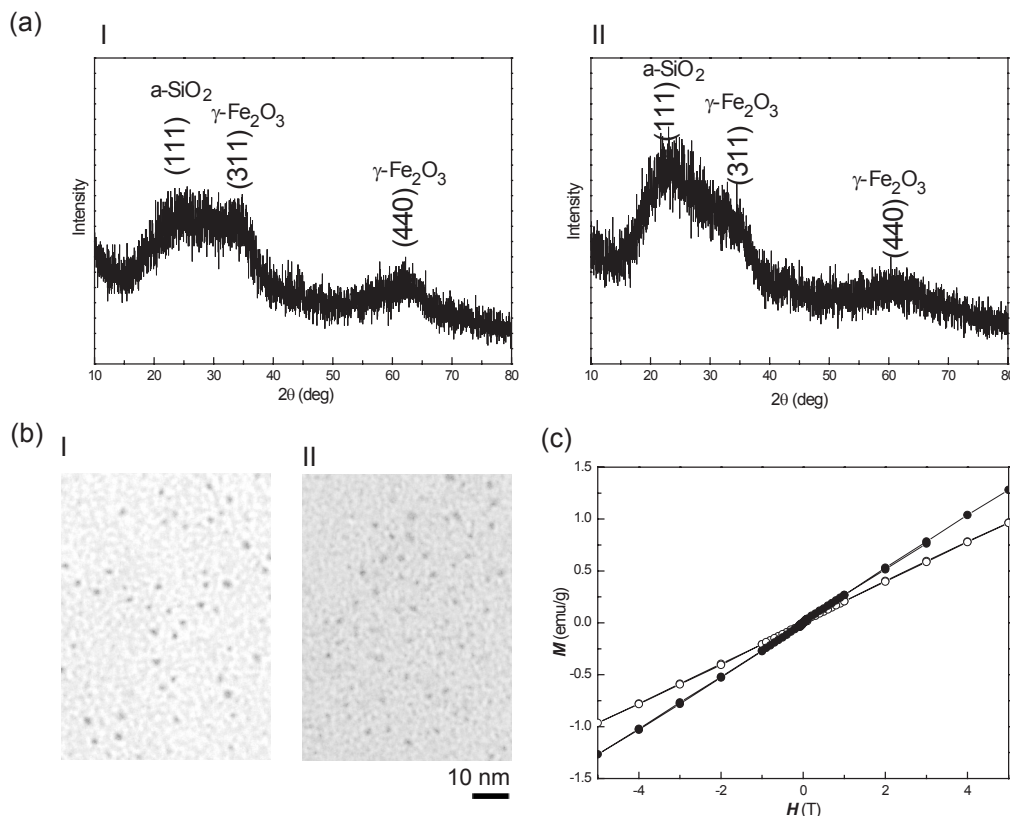
FIG. 2: The CuK \alpha XRD patterns of the unmodified NMPs (a-I) and amino-NMPs (a-II). TEM images of unmodified NMPs (b-I) and amino-NMPs (b-II). M - H curves for unmodified NMPs (○) and amino-NMPs (●).
