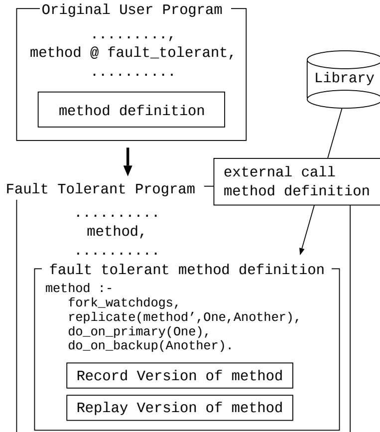
図 8.1: Converting original program
