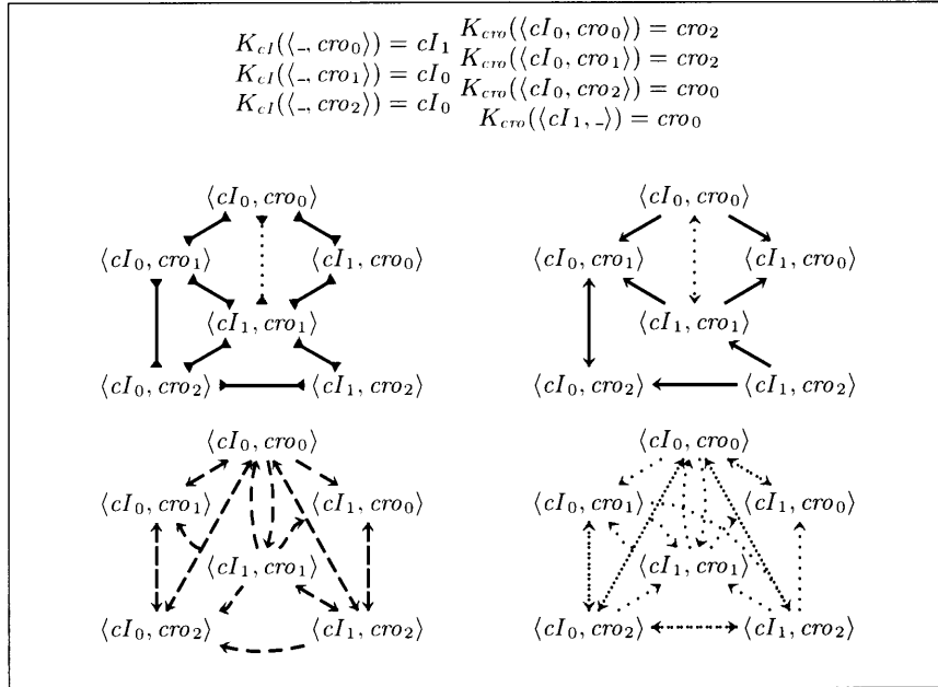
Fig. 7. \lambda -phage C/P game.
