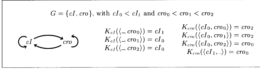
Fig. 5. Two-variable regulatory network for phage \lambda ( - is wildcard)
