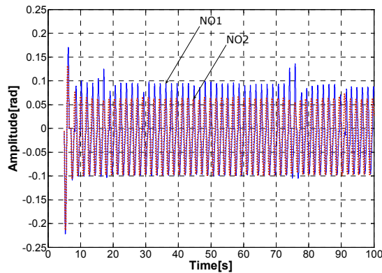
Fig. 9. The output of the neural oscillator coupled to the joints of the arm
