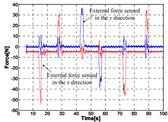
Fig. 8. The external forces measured by the force sensor in the x and y direction
