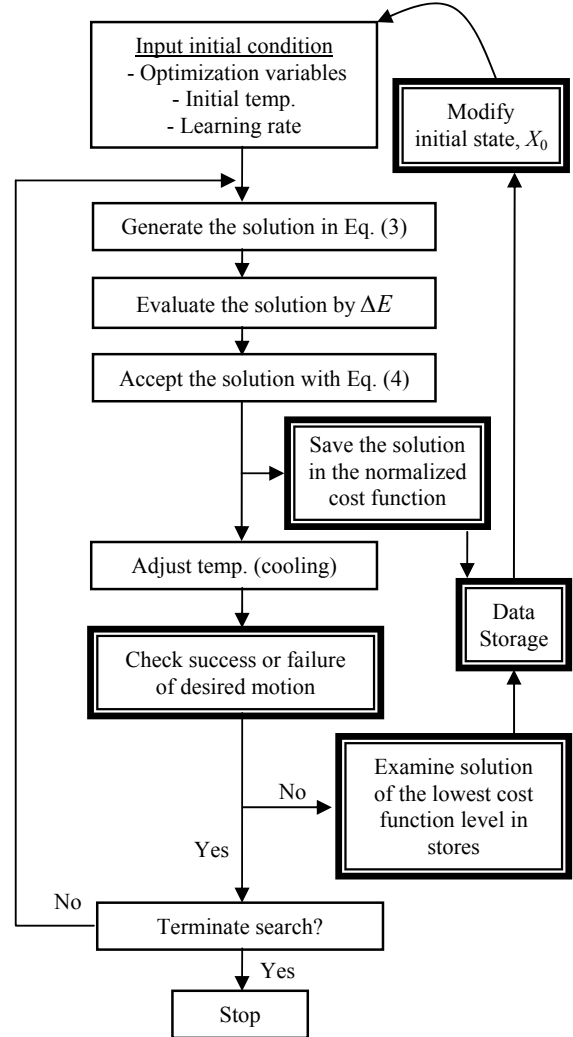
Fig. 3 Flowchart of the upgraded SA for task based parameter optimization.
