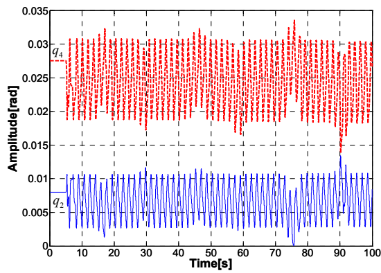
Fig. 10. The output of the first joint ( q_2 ) and the second joint ( q_4 )
