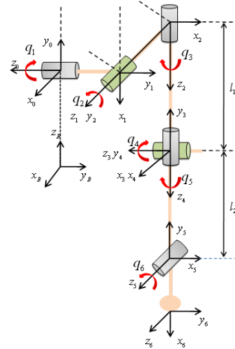
Fig. 6. Kinematic parameters of the robot arm
