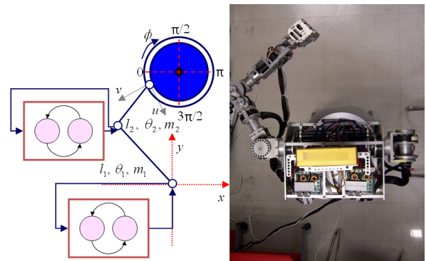
Fig. 4. (a) Schematic robot arm model and (b) real robot arm coupled with the neural oscillator for experimental test
