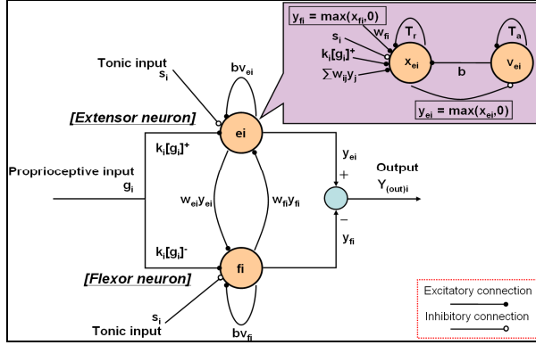
Fig. 1. Schematic diagram of Matsuoka Neural Oscillator
