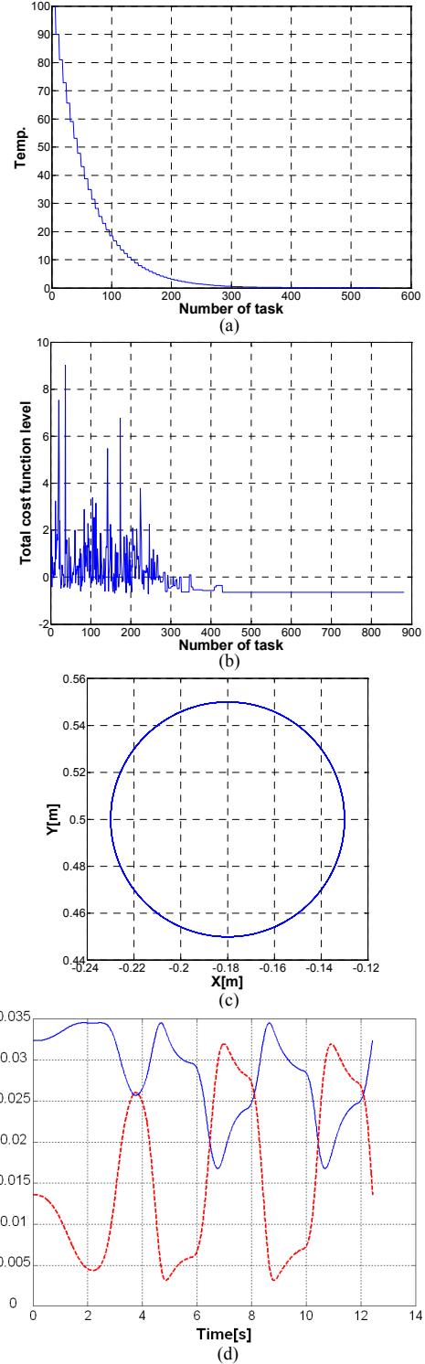
Fig. 5. (a) Temperature transition for cooling schedule, (b) A transition of total cost function level, (c) The end-effector trajectory of two-link arm (d) The output of joint angle. The red dash line is the first joint angle and the second joint angle is drawn by the blue thin line
