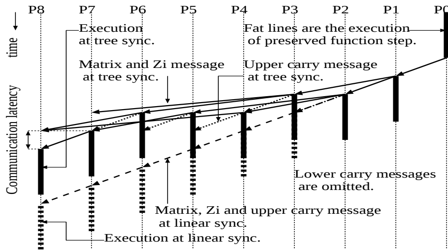
(a) Without response message.
