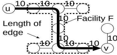
(a) Usual facility location.
