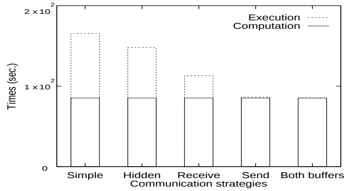
(c) Matrix size N = 1024 .
