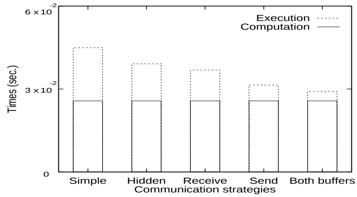
(b) Matrix size N = 64 .
