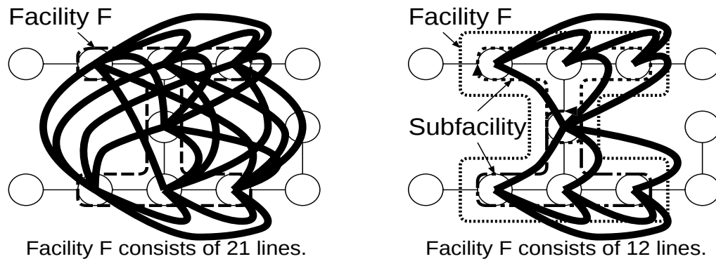
(a) Facility consists of complete connections. (b) Facility consists of two subfacilities.
