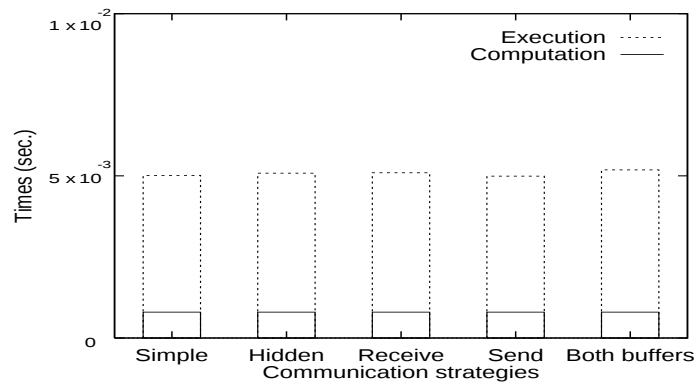
(a) Matrix size N = 8 .
