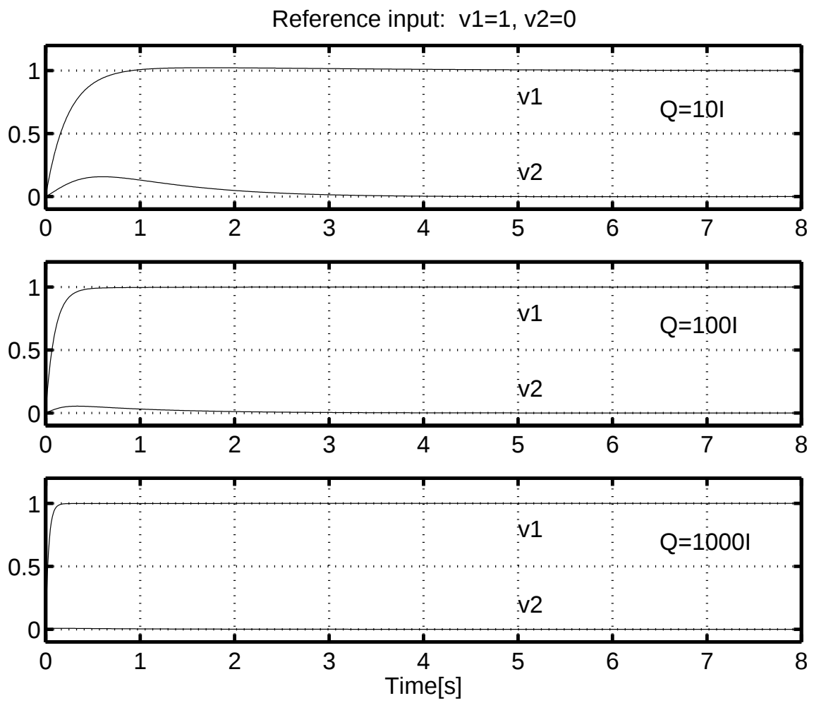
Fig 4.1: Step response for closed-loop system(minimum phase system)
