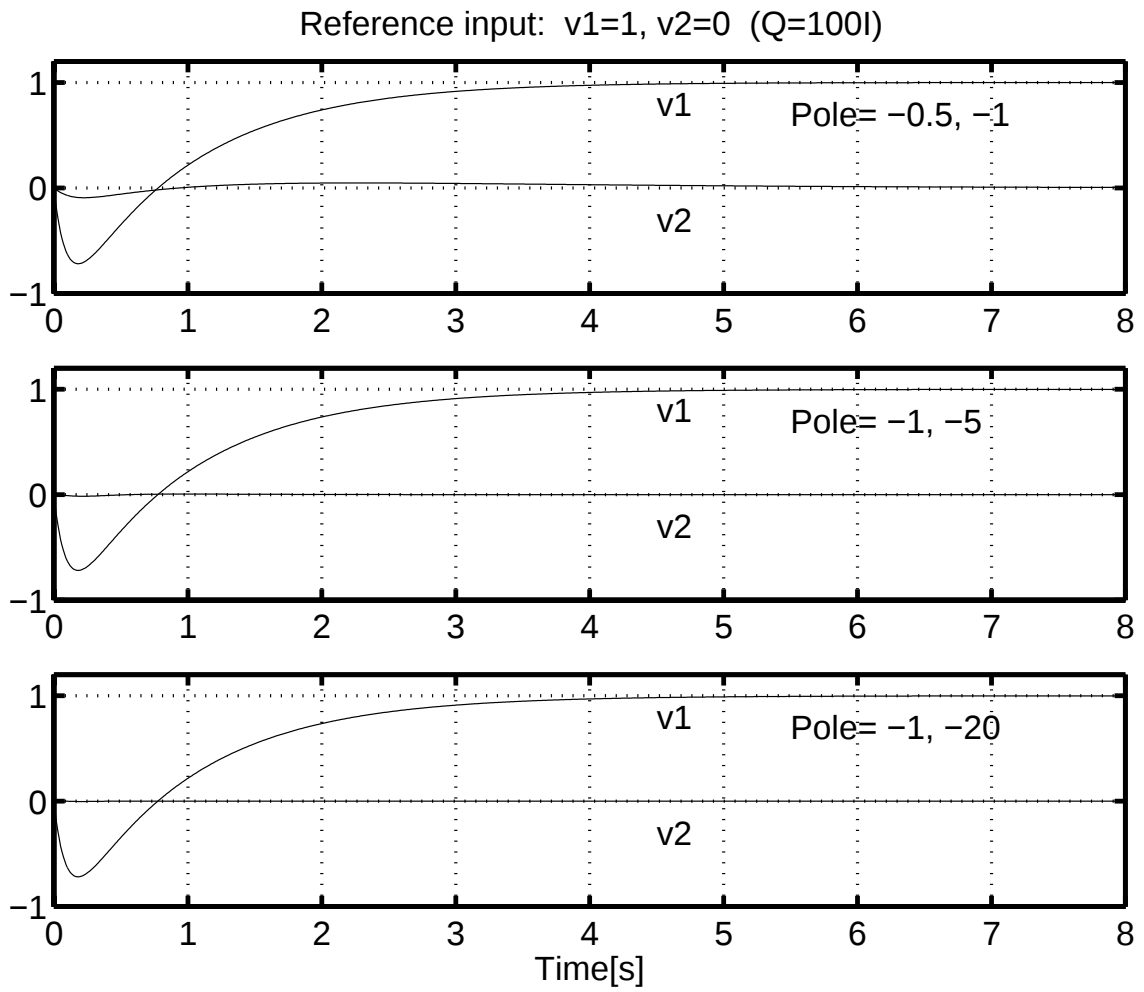
✕ 4.6: Step response for closed-loop system with pole placement(nonminimum phase system)
