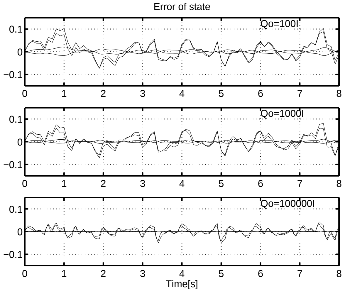
Fig 5.3: Error of state(full-order observer-based controller)
