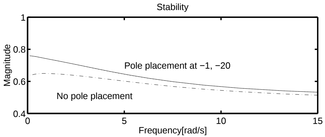
Figure 4.4: Stability margin; minimum phase system (—: Pole= -20, -1 , .....: Pole= -5, -1 , - · -: Pole= -0.5, -1 )
