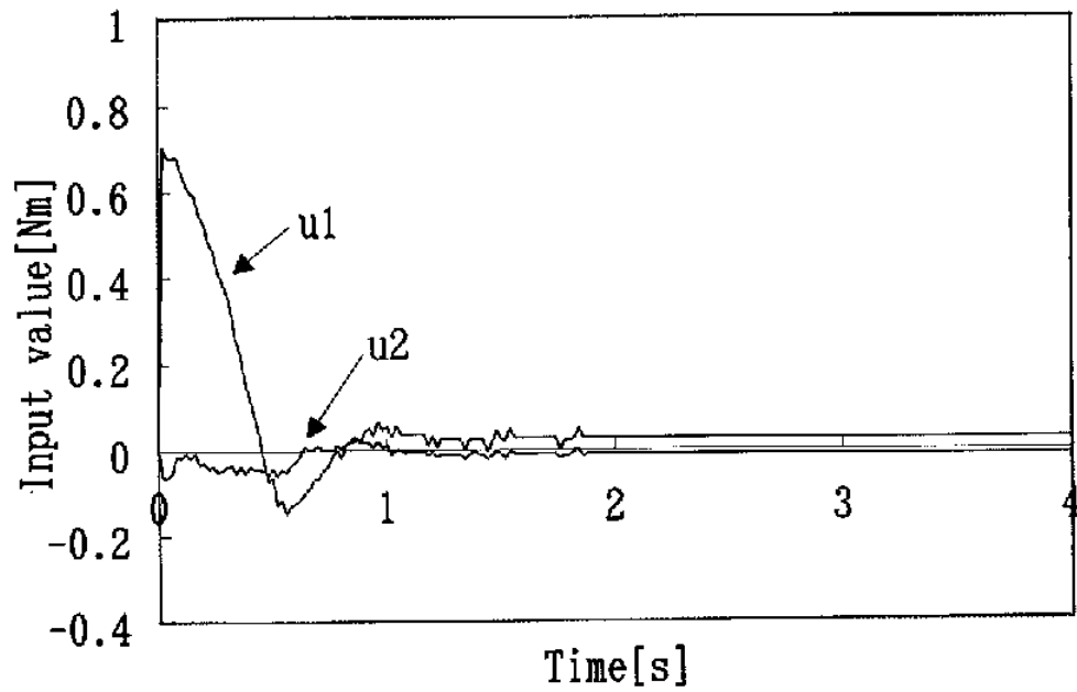
⊗ 3.5: Input value on motor
