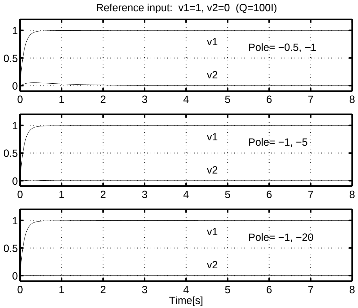
Fig 4.2: Step response for closed-loop system with pole placement(minimum phase system)
