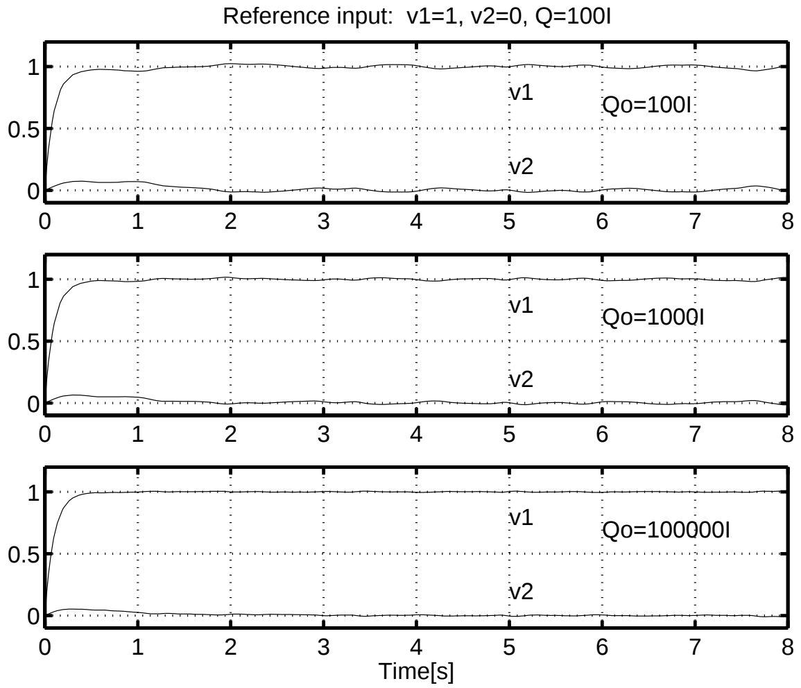
Fig 5.2: Step response for closed-loop system(full-order observer-based controller)
