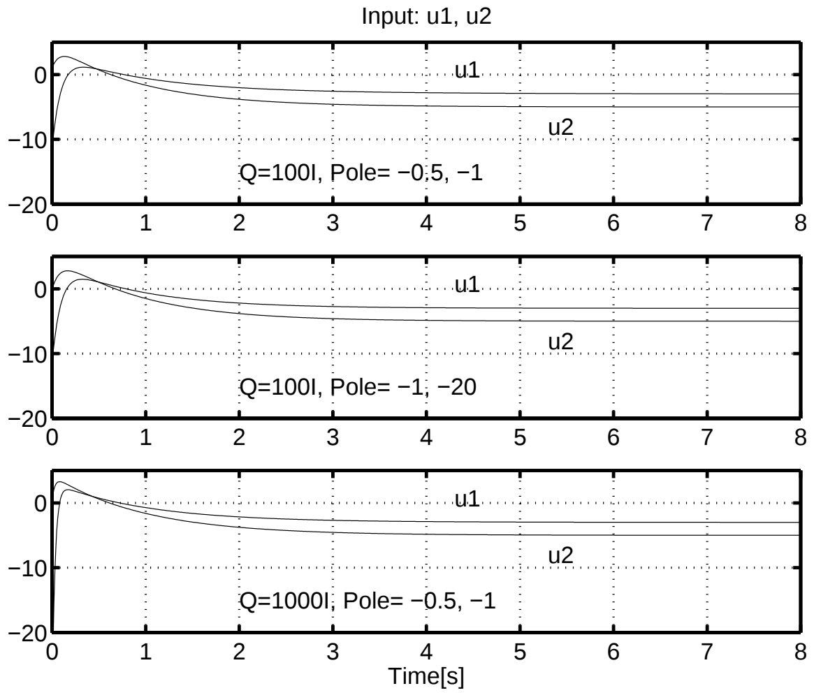
✎ 4.7: Input for closed-loop system with pole placement(nonminimum phase system)
