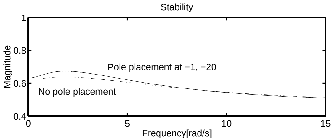
Fig 4.8: Stability margin; nonminimum phase system (—: Pole= -20, -1 , .....: Pole= -5, -1 , - · -: Pole= -0.5, -1 )
