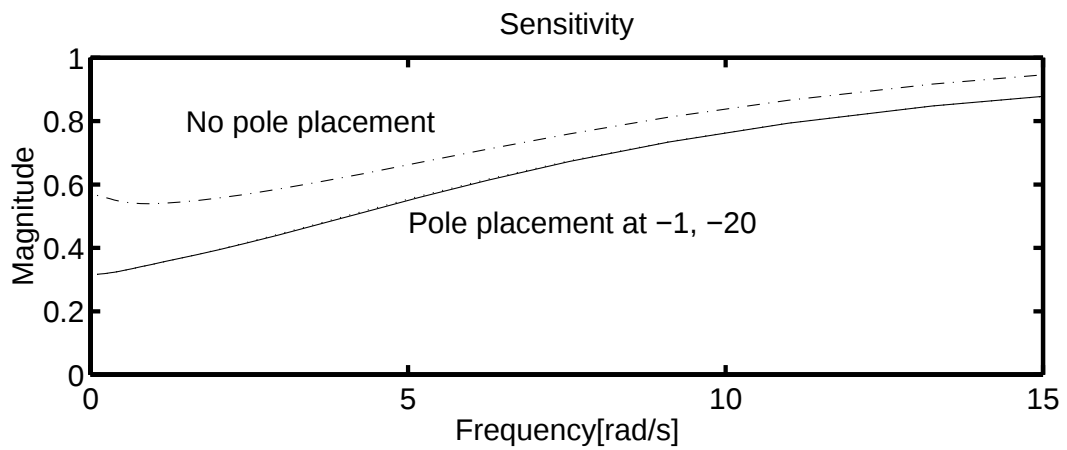
Figure 4.5: Sensitivity margin; minimum phase system (—: Pole= -20, -1 , .....: Pole= -5, -1 , - · -: Pole= -0.5, -1 )
