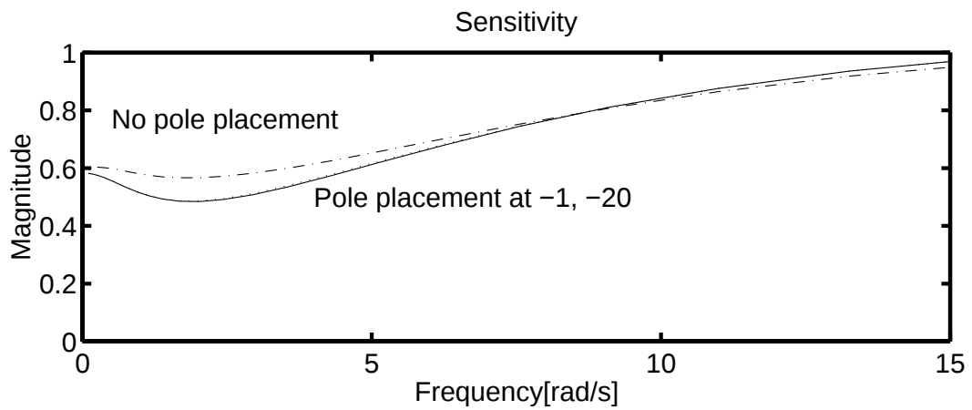
Fig 4.9: Sensitivity margin; nonminimum phase system (—: Pole= -20, -1 , .....: Pole= -5, -1 , - · -: Pole= -0.5, -1 )
