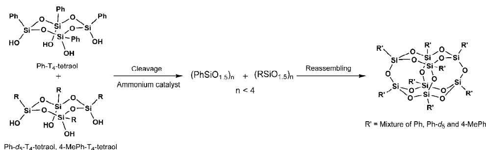
Scheme 2. Reaction mechanism in the formation of T 8 from T 4 -tetrol using ammonium catalysts
