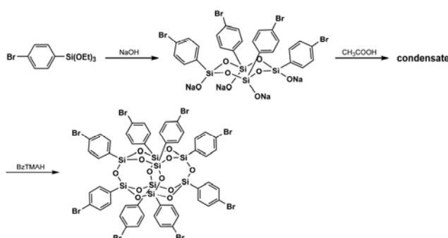
Scheme 3. Synthesis of octa(4-bromophenyl)octasilsesquioxane
