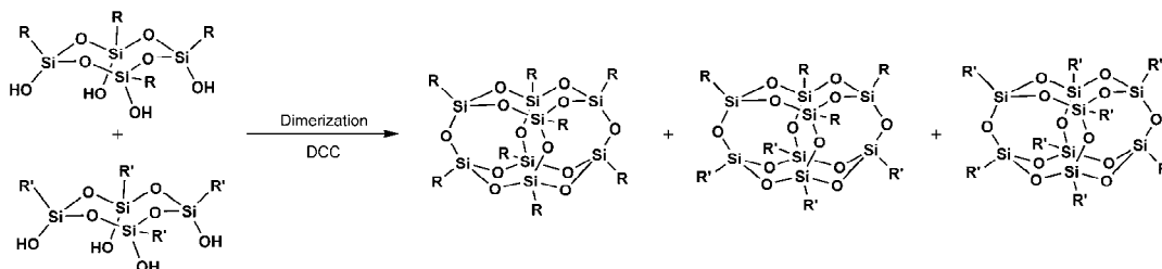
Scheme 4. Synthesis of T 8 cages from co-condensation of Ph-T 4 -tetrol and Ph- d 5 -T 4 -tetrol by DCC
