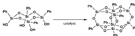
Scheme 1. Synthesis of \text{T}_8 cage from all- cis - \text{Ph-T}_4 -tetrol
