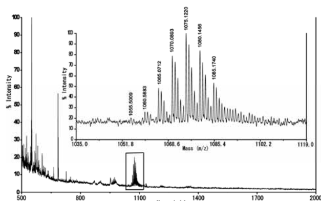
Figure 2. Mass spectrum of the product cages from the mixture of Ph- and Ph- d 5 -T 4 -tetrol.
