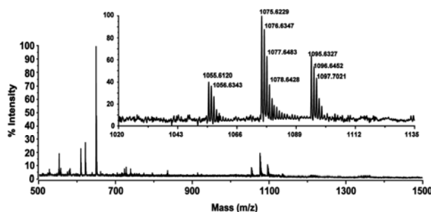
Figure 3. Mass spectrum of the product T 8 cages from the mixture of Ph- and Ph- d 5 -T 4 -tetrol.
