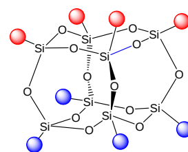
Figure 1. Structure of \text{C}_{4v} -symmetry \text{T}_8 Cage.
