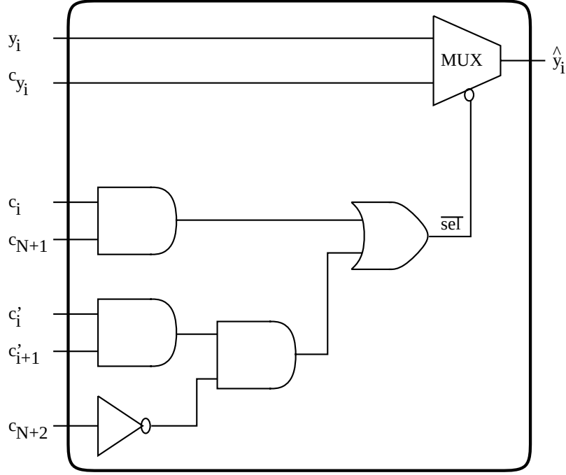
Figure 6.7: The circuit for correcting the erroneous output y_i .
