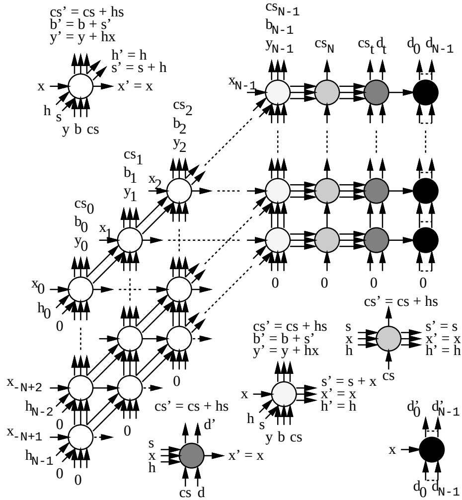
(a) Dependence graph for FIR filtering with fault tolerance.
