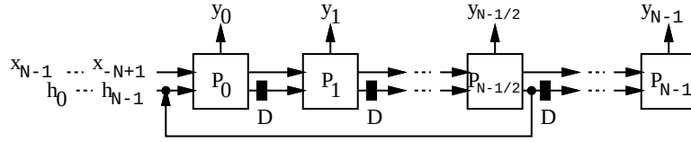
(b) A systolic FIR filter.
