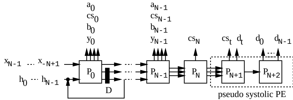
(b) A fault tolerant FIR filter.
