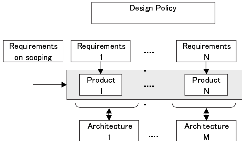
Figure 3.6: Product-line Scoping
