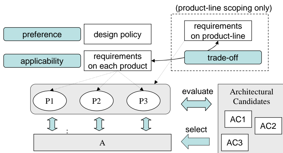
Figure 1.4: Architectural Design
