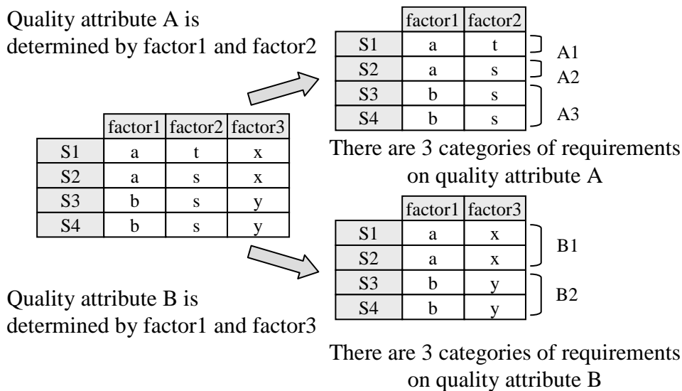
Figure 4.5: Separate Aspects
