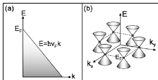
Fig. 13. (a) Linear dispersion expected for graphene. (b) Point-like Fermi surface and cone-like dispersion. The figure is taken from Ref. [29].
