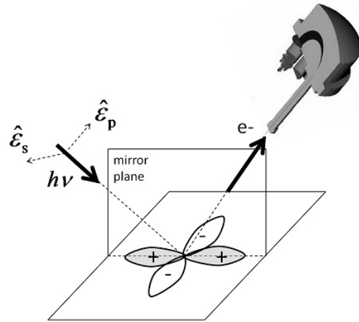
Fig. 4. Photoemission from a d_{x^2-y^2} orbital on the mirror plane (the detector is also located on the mirror plane).
