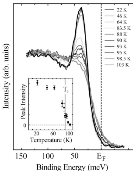
Fig. 10. Temperature-dependent spectra from optimally doped Bi2212 ( T_c = 91 K), angle integrated over a narrow cut at (\pi,0) . Inset: superconducting-peak intensity with respect to temperature. The figure is taken from Ref. [26].
