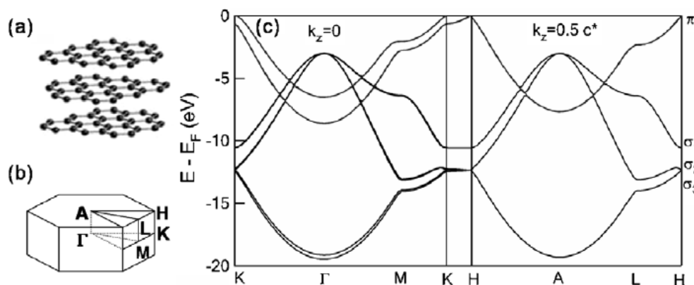
Fig. 12. (a) Crystal structure of graphite. (b) BZ of graphite. (c) \pi bands (touching the Fermi level) and \sigma bands along the high symmetry directions of graphite. The figure is taken from Ref. [29].
