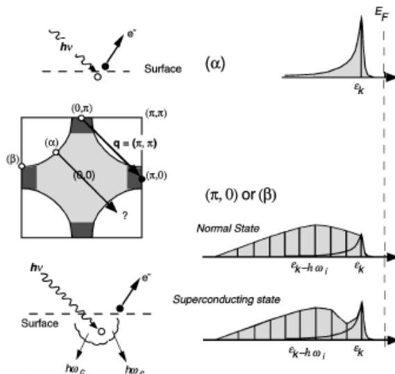
Fig. 11. Photoemission line shape for weak coupling ( \alpha ) and strong coupling ( \beta ), i.e. near (\pi,0) . Phase-space consideration for a coupling to (\pi,\pi) resonant mode results in the anisotropy. The figure is taken from Ref. [27].
