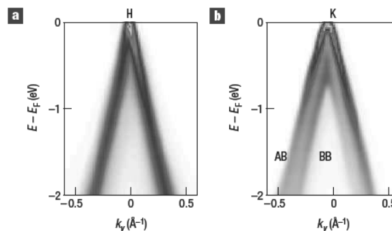
Fig. 14. Dispersions measured near BZ H and K points. (a) Linear dispersion near BZ H point implying the presence of the massless Dirac fermion. (b) Quadratic dispersion (near the Fermi level) near BZ K point implying the quasiparticle with the finite mass. The \pi bands are split into bonding (BB) and anti-bonding (AB) bands. The figure is taken from Ref. [30].
