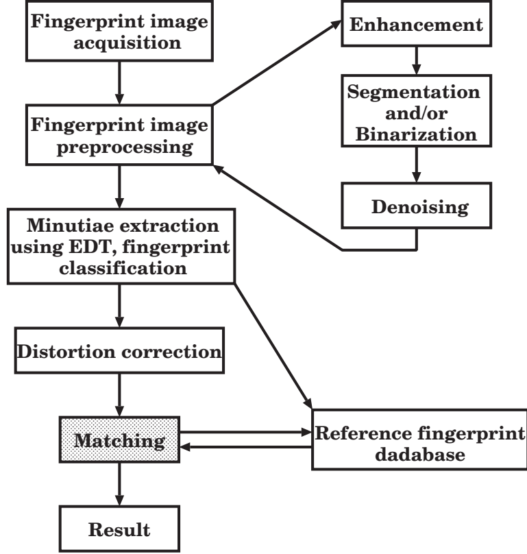
Figure 8.2: A flowchart showing different phases of fingerprint analysis. The highlighted block shows our work in this chapter.
