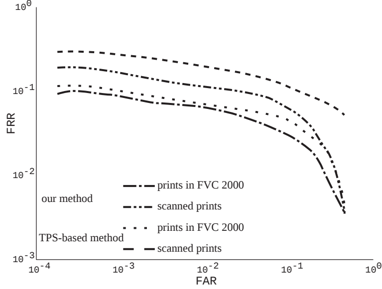
Figure 8.8: ROC curves on FVC2000 DB and scanned fingerprints obtained with the proposed method and the algorithm in [5].
