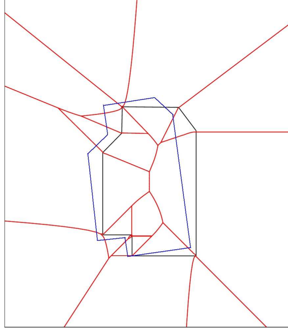
Figure 8.7: Intersection of Voronoi-cell \text{Vor}(P) with Q . P is colored black; its Voronoi edges are red. Q is colored blue.
