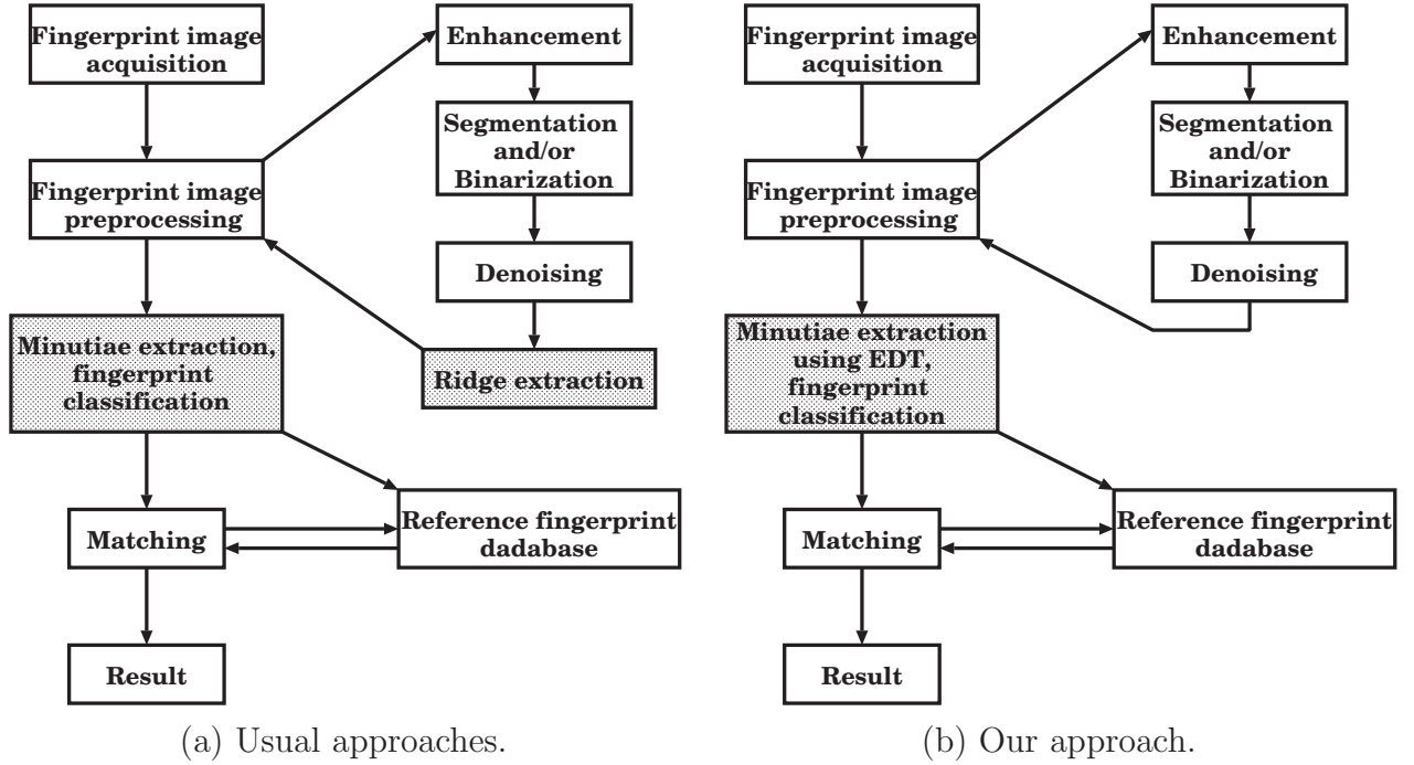
Figure 6.3: Two flowcharts showing the different phases in fingerprint analysis taken by (a) usual approaches and (b) our method. In (b) the highlighted modules show the area of our work.
