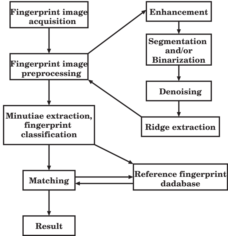
Figure 1.1: A flowchart showing different phases of fingerprint analysis.
