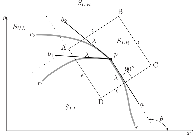
Figure 8.3: Minutia detail and defining \epsilon -square box with regard to a bifurcation minutia at p .
