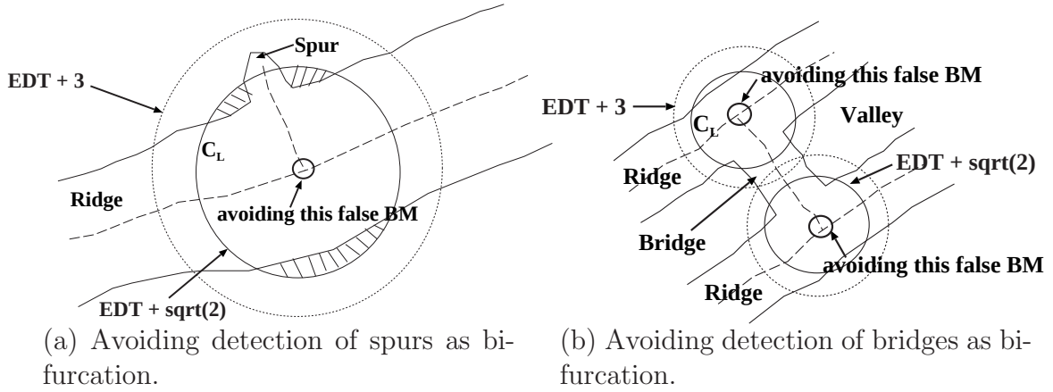
Figure 6.6: Finding correct bifurcation minutiae(BM) by avoiding spurs and bridges.
