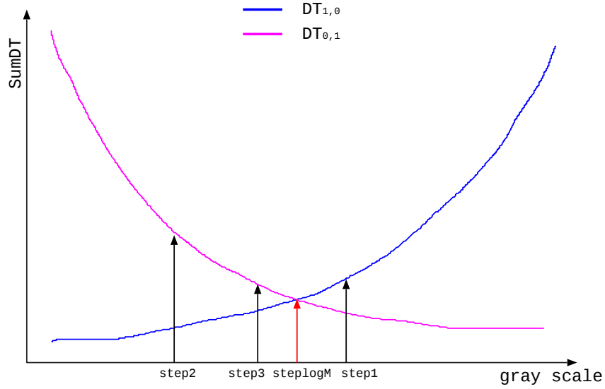
Figure 4.6: Diagram of binarization algorithm.
