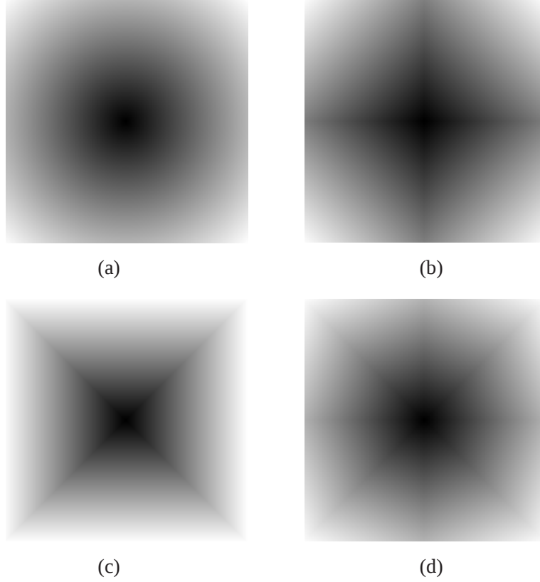
Figure 3.1: Four commonly used distance metrics C measuring the distance from the center of the image: (a) Euclidean metric, Equation 3.3; (b) city block metric, Equation 3.4; (c) chessboard metric, Equation 3.5; (d) a quasi-Euclidean metric, Equation 3.6
