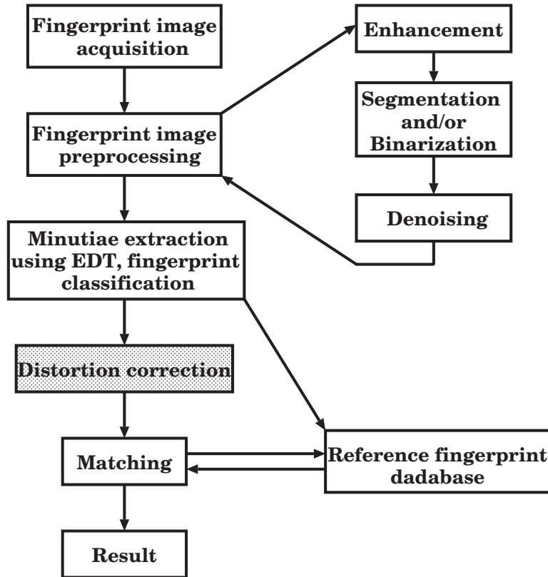
Figure 7.1: A flowchart showing different phases of fingerprint analysis. The highlighted block shows our work in this chapter.
