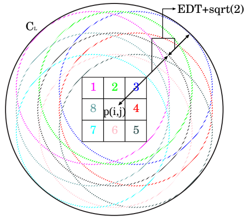
(b) Circles formed by the EDT value; the circle C_L is the smallest radius circle covering all the 9 EDT circles (shown dotted).
