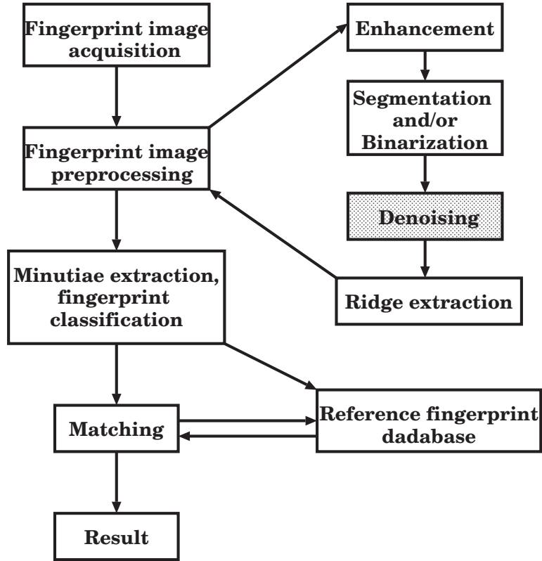
Figure 5.1: A flowchart showing different phases of fingerprint analysis. The highlighted block shows our work in this chapter.
