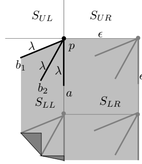
Figure 8.4: Bifurcation polygon (case 1).
