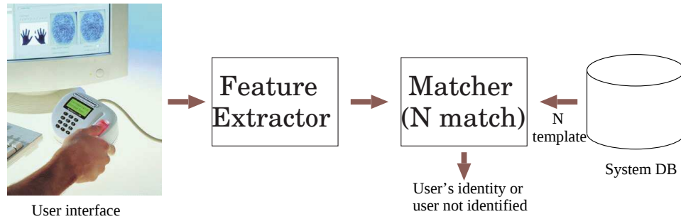
Figure 2.3: A fingerprint identification system.
