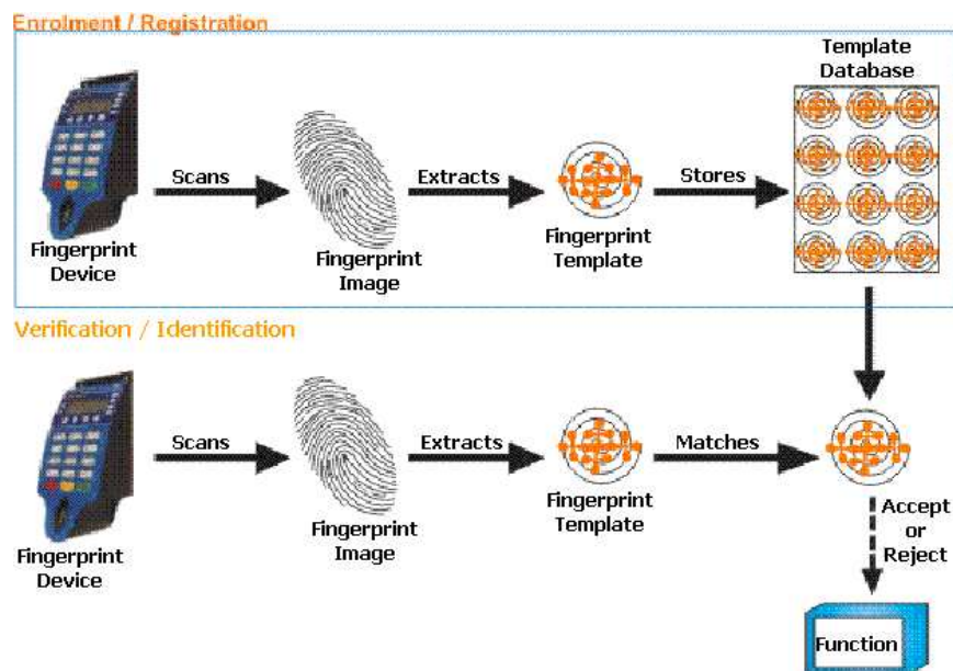
Figure 2.1: A fingerprint recognition system.
