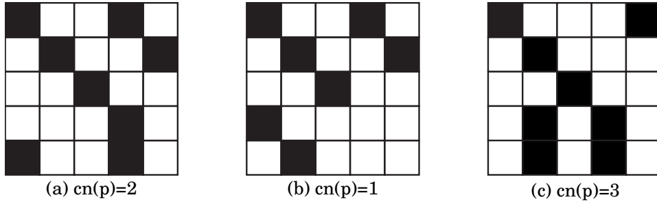
Figure 6.2: (a) intra-ridge pixel; (b) termination minutia; (c) bifurcation minutia.
