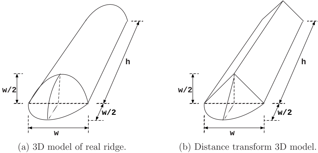
Figure 5.8: Diagrams of the 3D model.
