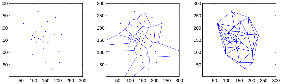
Figure 7.2: (left) A set of points, (middle) its Voronoi diagram, and (right) its Delaunay triangulation.
