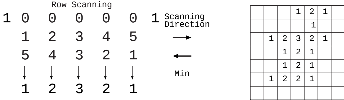
Figure 3.2: Compute horizontal distance by bidirectional scanning and take minimum of each such distance.
